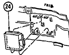
MODULE ASM TO CARPET SUPPORT
