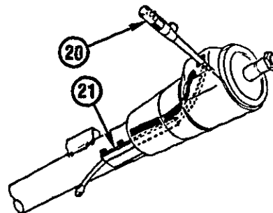
VACUUM RELEASE VALVE TO BRAKE PEDAL
