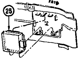
MODULE ASM TO CARPET SUPPORT
