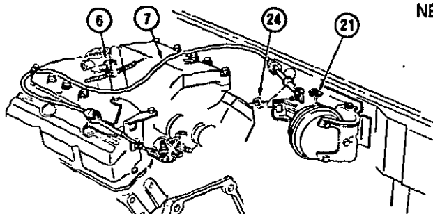
CABLE ASM-CRUISE CONTROL
